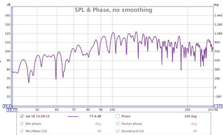
SPL and Phase
